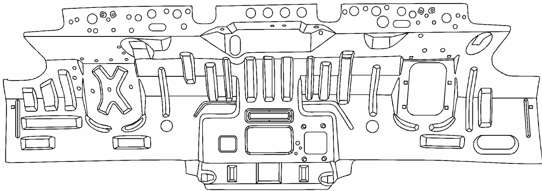
PSMP08 Front Cabin Floor Assy.
