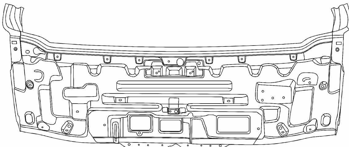
PSMP94 Front Panel Inner Assey.
