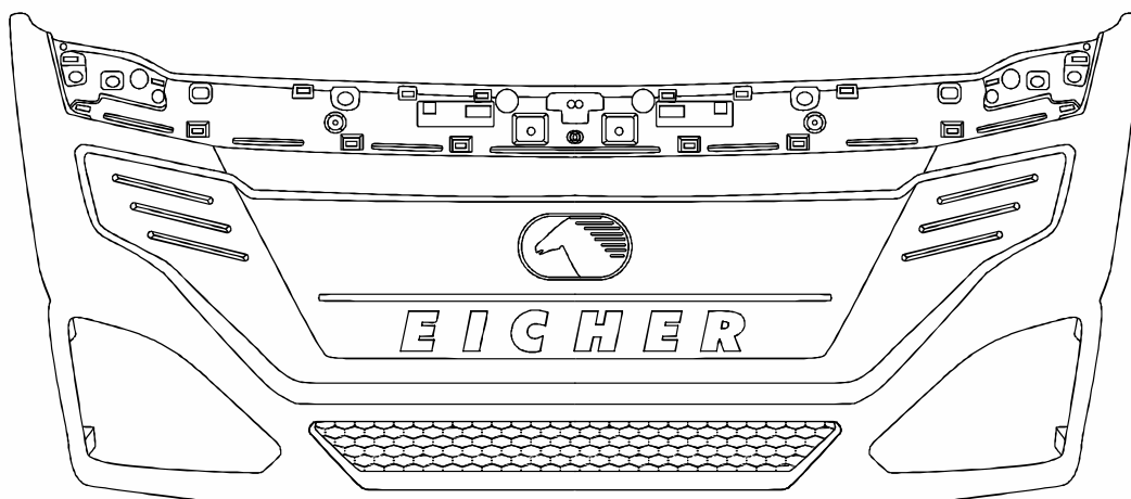
PSMP93 Front Show Metal (2059)
