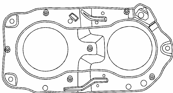
PSMP16 Front Headlight Housing O/M - RH/LH
