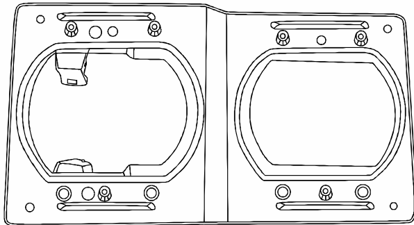
PSMP58 Front Headlight Housing - N/M - RH/LH
