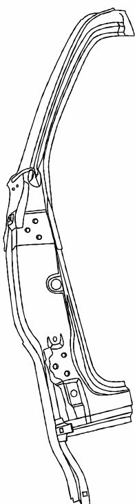
PSMP78 Front Pro - Pillar Assy. - RH/LH
